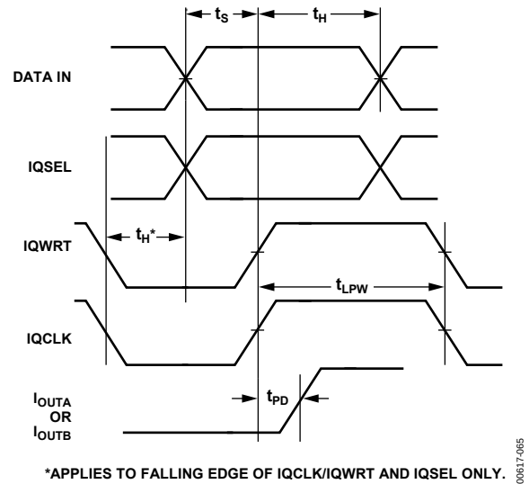
Figure 65. 5 V Only Interleaved Mode Timing
