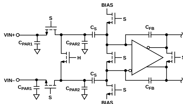
Figure 46. Switched-Capacitor Input
