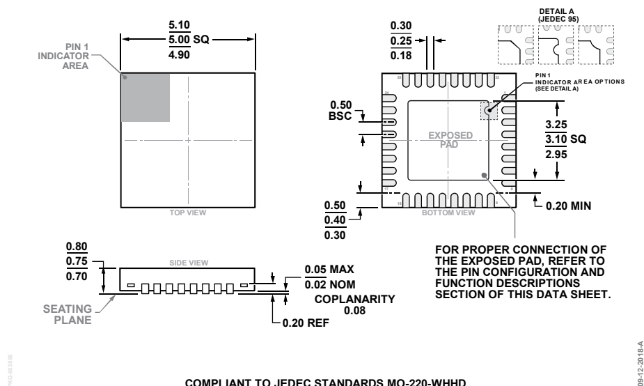
COMPLIANT TO JEDEC STANDARDS MO-220-WHHD Figure 43. 32-Lead Lead Frame Chip Scale Package [LFCSP] 5 mm x 5 mm Body and 0.75 mm Package Height (CP-32-7) Dimensions shown in millimeters
