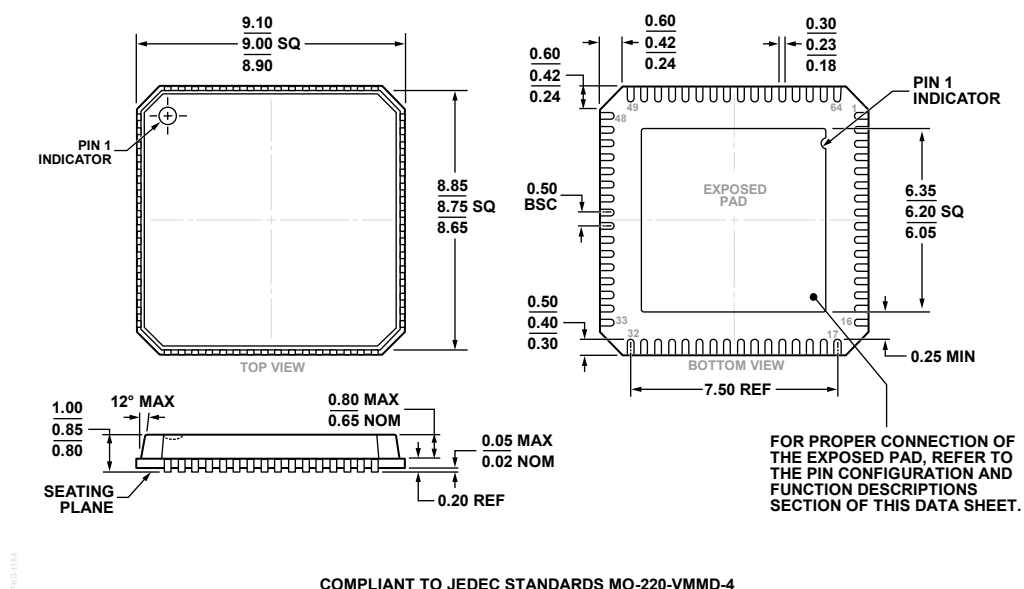
Figure 75. 64-Lead Lead Frame Chip Scale Package [LFCSP_VQ] 9 mm x 9 mm Body, Very Thin Quad CP-64-4 Dimensions shown in millimeters
