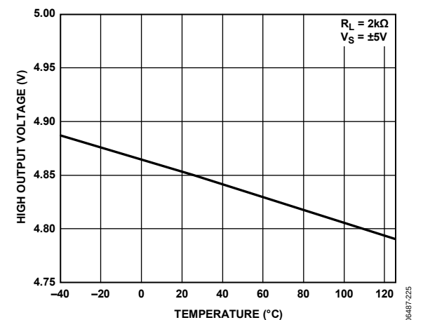
Figure 26. High Output Voltage, V_{OH} vs. Temperature, V_S = \pm 5\text{ V}
