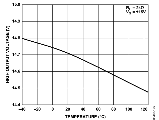
Figure 25. High Output Voltage, V_{OH} vs. Temperature, V_S = \pm 15\text{ V}
