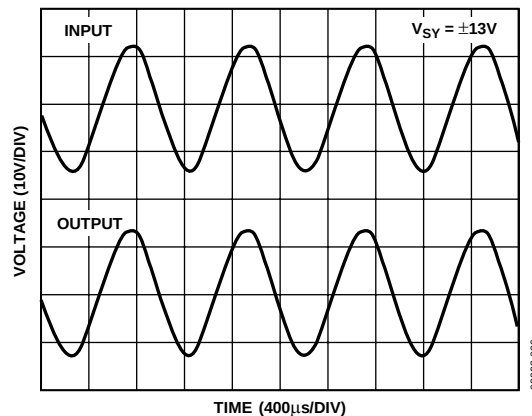
Figure 29. No Phase Reversal
