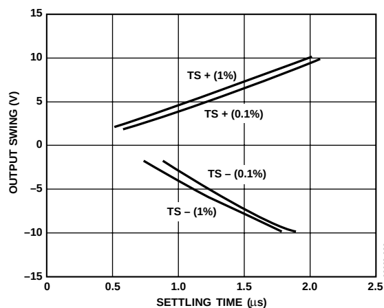
Figure 30. Output Swing and Error vs. Settling Time
