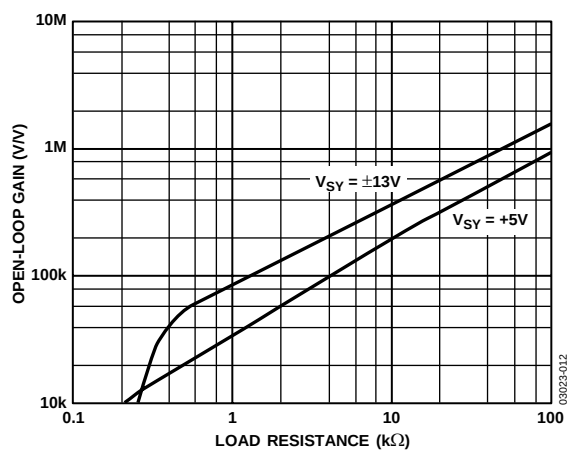
Figure 12. Open-Loop Gain vs. Load Resistance
