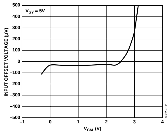
Figure 11. Input Offset Voltage vs. V_{CM}
