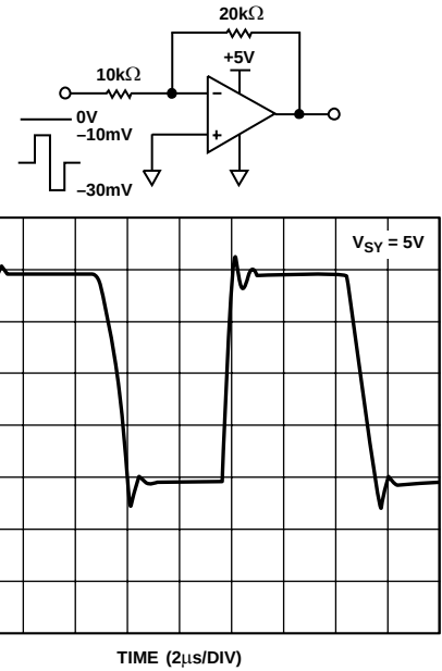
Figure 43. Gain-of-Two Inverter Response to 20 mV Step, Centered 20 mV below Ground
