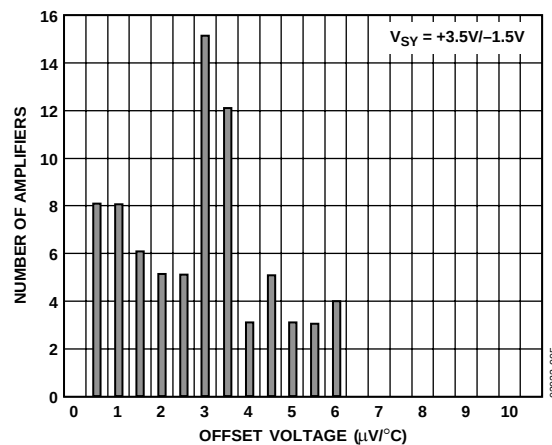
Figure 5. Offset Voltage Drift
