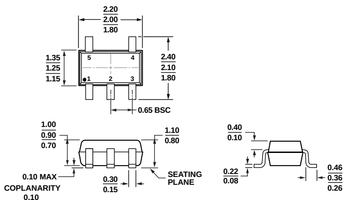
Figure 50. 5-Lead Plastic Surface-Mount Package [SC70] (KS-5)
