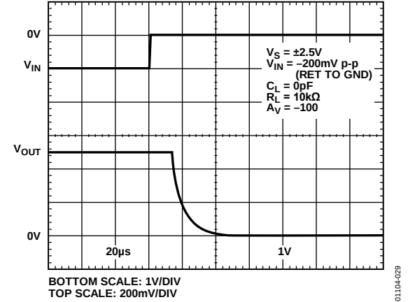
Figure 29. Positive Overvoltage Recovery
