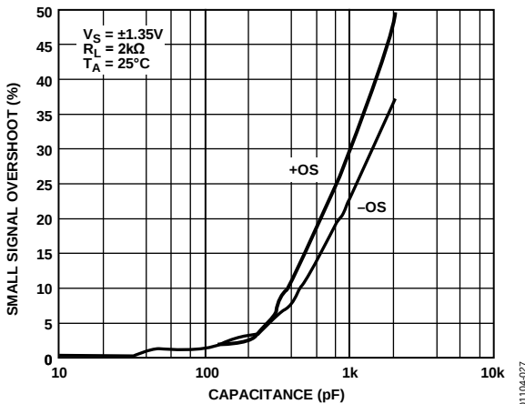
Figure 27. Small Signal Overshoot vs. Load Capacitance
