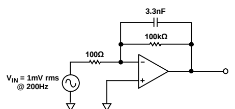
Figure 59. Reducing Autocorrection Clock Noise Using a Feedback Capacitor
