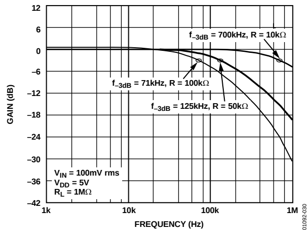
Figure 30. -3dB Bandwidths
