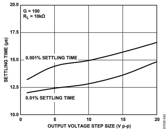
Figure 40. Settling Time vs. Step Size, G = 100
