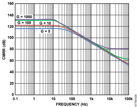
Figure 28. CMRR vs. Frequency, RTI, 1 k \Omega Source Imbalance
