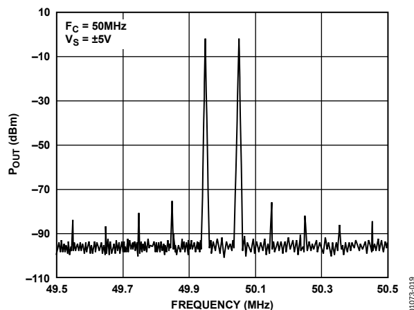
Figure 19. Intermodulation Distortion
