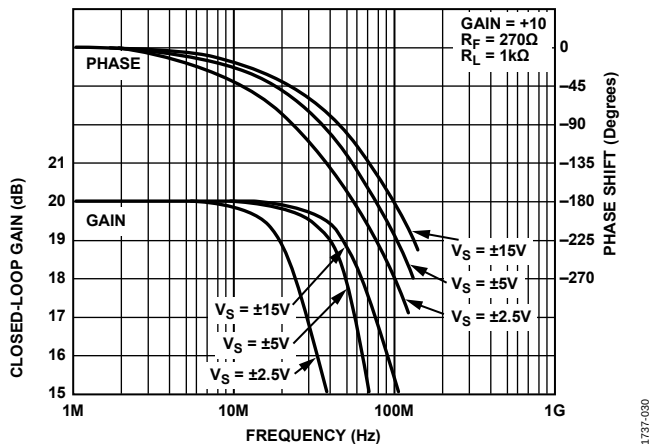
Figure 32. Closed-Loop Gain and Phase Shift vs. Frequency, G = +10 , R_L = 1k\Omega
