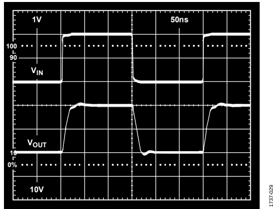
Figure 31. Large Signal Pulse Response, Gain = +10, R_F = 442\Omega , R_L = 400\Omega , V_S = \pm 15V
