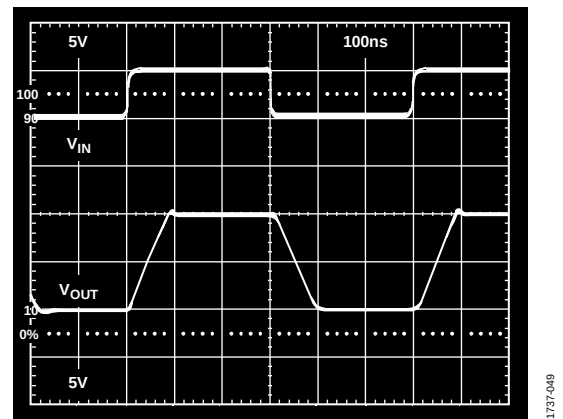
Figure 51. AD810 Driving a 1000 pF Load, Gain = +2, R_F = 750 \Omega , R_S = 11 \Omega , R_L = 10 \text{ k}\Omega
