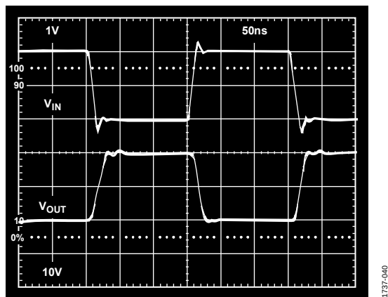
Figure 42. Large Signal Pulse Response, Gain = -10, R_F = 442\ \Omega , R_L = 400\ \Omega , V_S = \pm 15\ V
