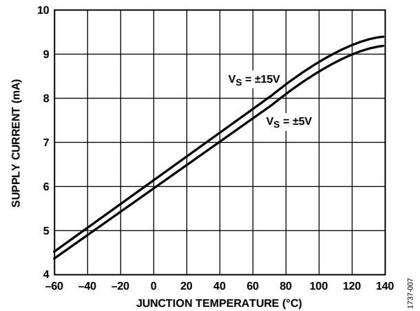
Figure 9. Supply Current vs. Junction Temperature
