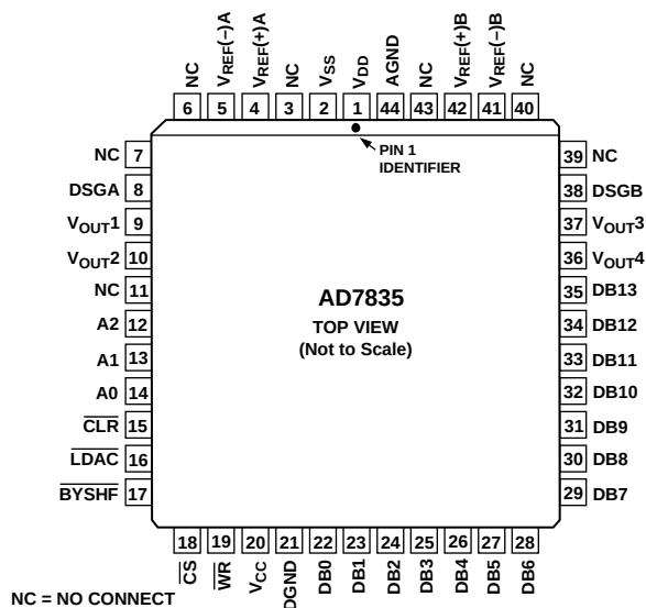
Figure 8. AD7835 PLCC Pin Configuration
