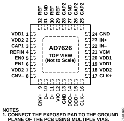
Figure 4. Pin Configuration
