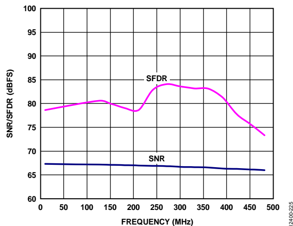
Figure 36. SNR/SFDR vs. Analog Input Frequency ( f_{IN} ); f_{IN} < 500\text{ MHz}; \text{Buffer Control 1} = 3.0\times
