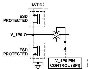
Figure 73. V_1P0 Input/Output
