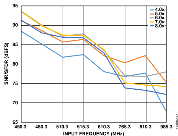
Figure 85. Buffer Current Sweeps, AD6674-500 (SFDR vs. Input Frequency and I_{BUFF} ); 450 MHz < f_{IN} < 1000 MHz; Front-End Network Shown in Figure 74
