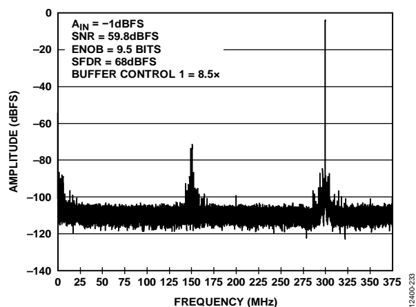
Figure 33. Single Tone FFT with f_{IN} = 1950.3\text{ MHz}
