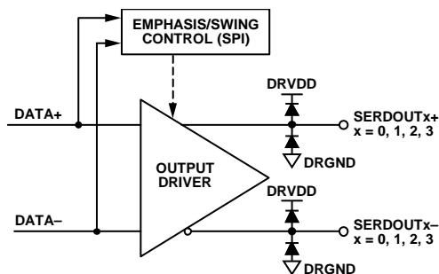
Figure 66. Digital Outputs
