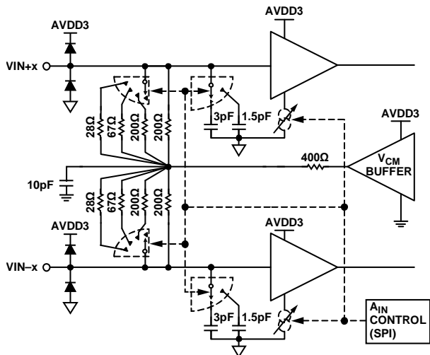
Figure 63. Analog Inputs
