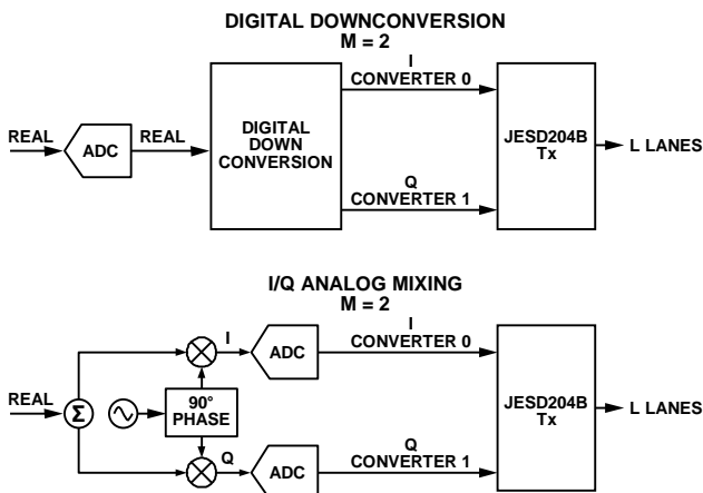
Figure 139. I/Q Transport Layer Mapping
