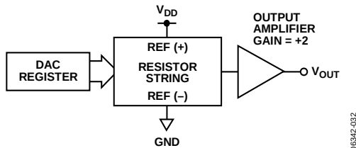
Figure 52. DAC Architecture
