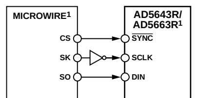
Figure 59. AD5623R/AD5643R/AD5663R to MICROWIRE Interface
