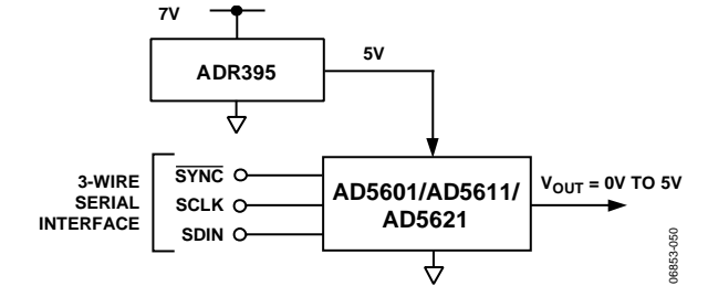
Figure 51. ADR395 as Power Supply to the AD5601/AD5611/AD5621 Some recommended precision references for use as supplies to the AD5601/AD5611/AD5621 are listed in Table 7.
