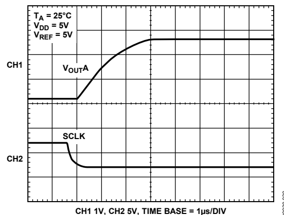
Figure 20. Half-Scale Settling ( \frac{1}{4} to \frac{3}{4} Scale Code Change)
