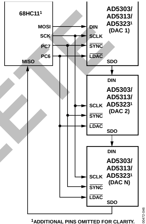
Figure 46. Daisy-Chain Mode
