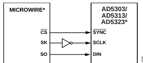
Figure 38. AD5303/AD5313/AD5323 to MICROWIRE Interface
