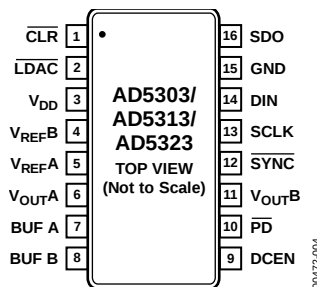
Figure 6. Pin Configuration
