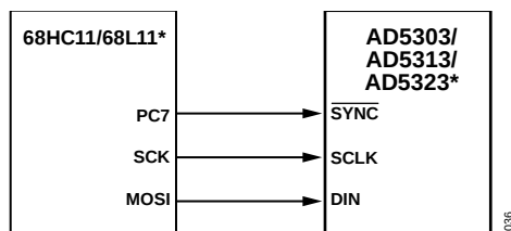
Figure 36. AD5303/AD5313/AD5323 to 68HC11/68L11 Interface
