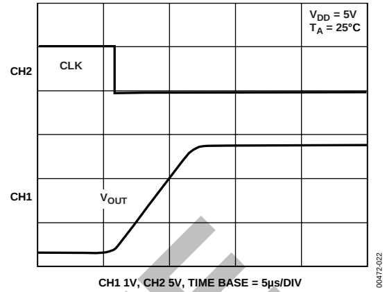
Figure 22. Half-Scale Settling ( 1/4 to 3/4 Scale Code Change)
