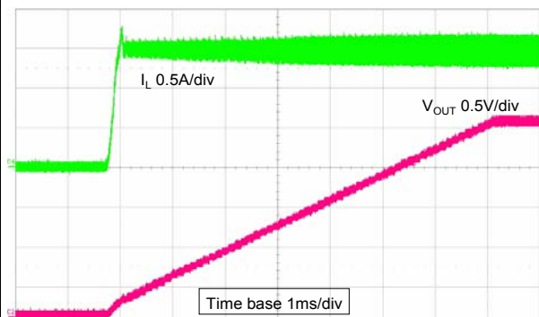
Figure 31. Soft-start
