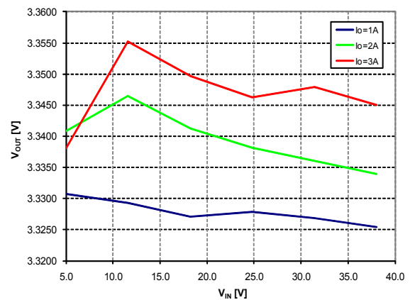
Figure 29. Line regulation
