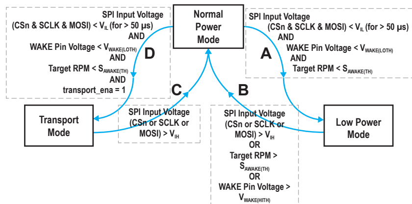
Figure 3: Operating Mode State Diagram
