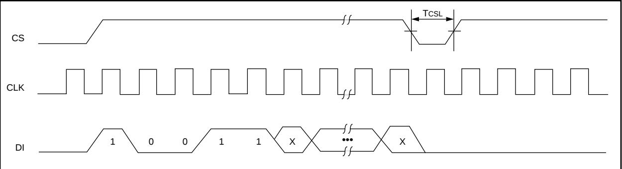
FIGURE 3-5: EWEN TIMING
