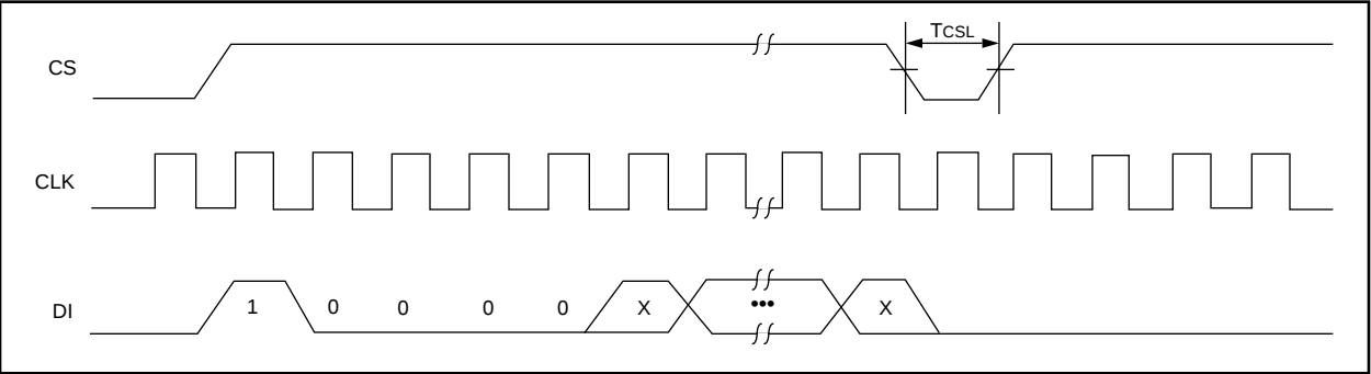
FIGURE 3-4: EWDS TIMING
