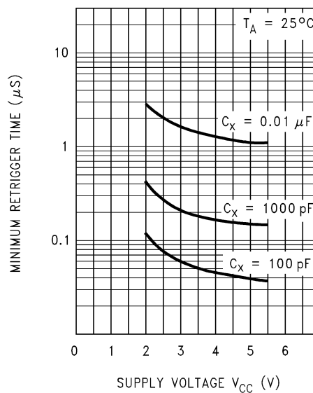
t RR *V CC Characteristics (Typ.)
