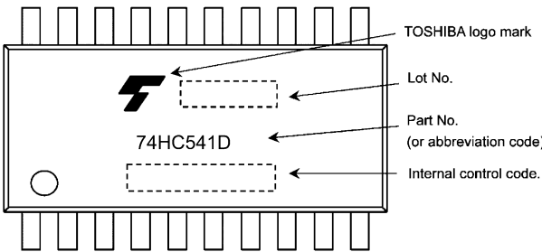
74HC541D
