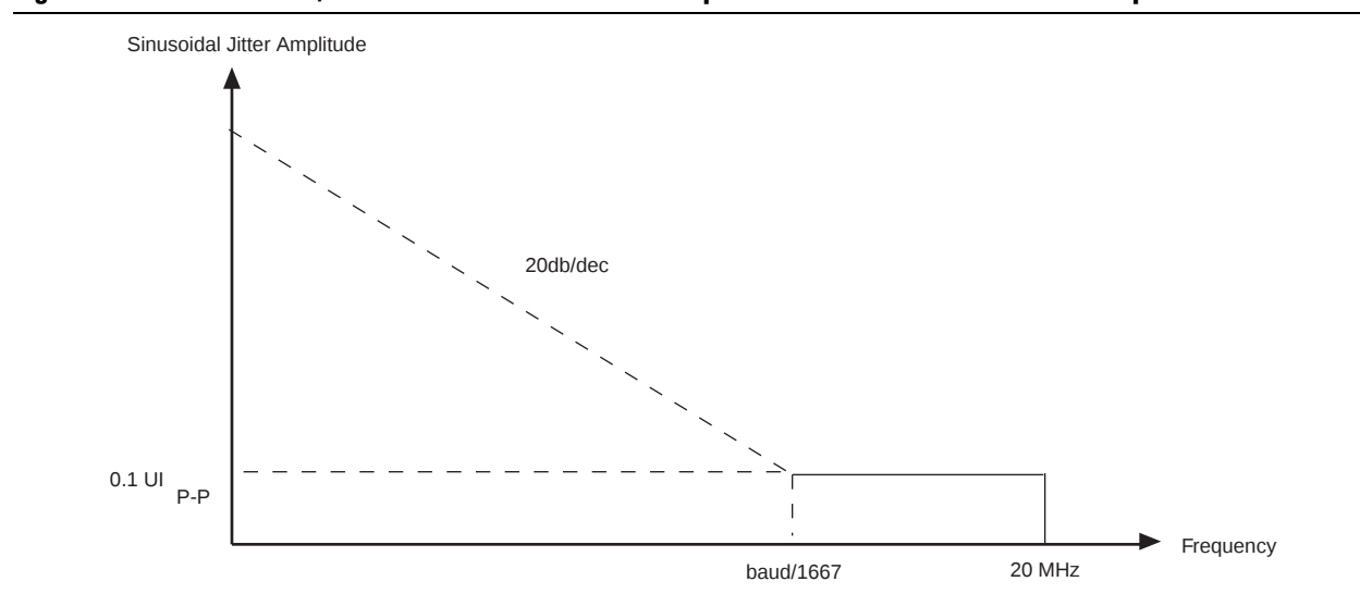
Figure 2-3. LVDS Soft-CDR/DPA Sinusoidal Jitter Tolerance Specification for a Data Rate < 1.25 Gbps
