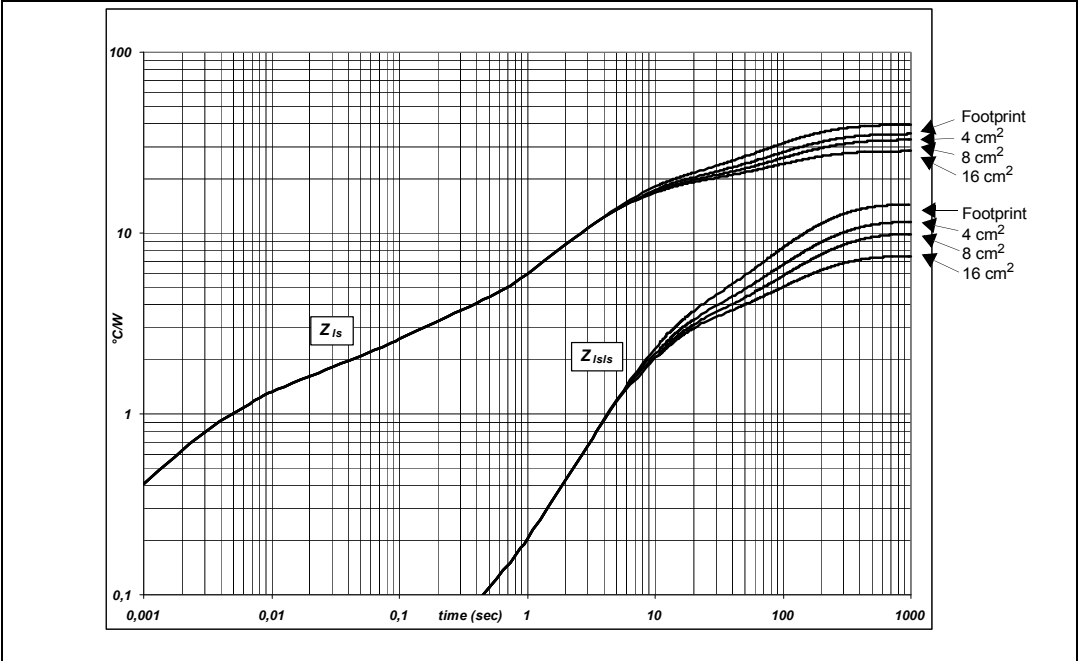
Figure 42. Thermal fitting model of an H-bridge in MultiPowerSO-30
