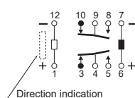
2 coil latching
