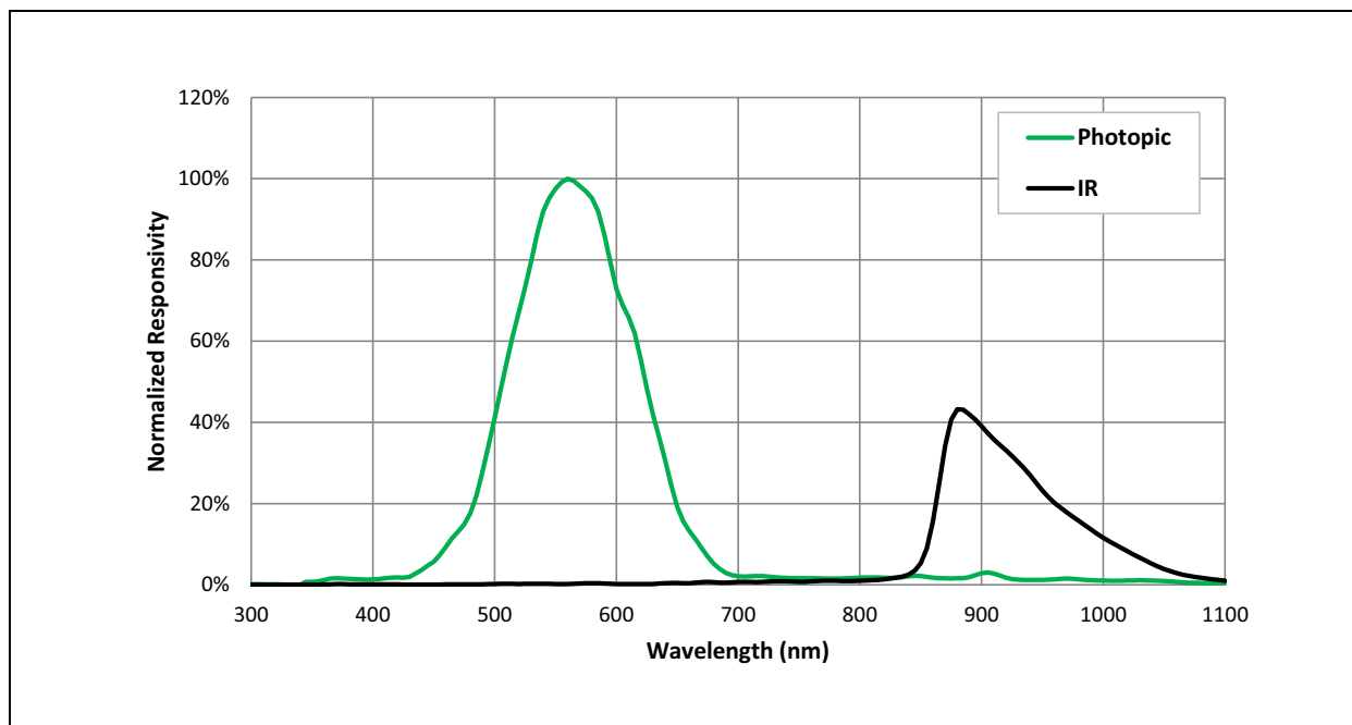
Figure 11: Spectral Responsivity
