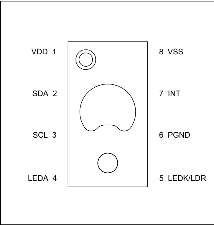
Figure 3: Pin Diagram of TMD2725
