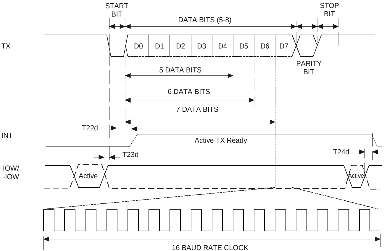
Transmit timing
