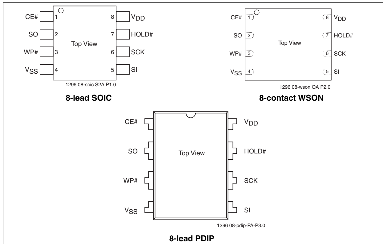
FIGURE 2-1: PIN ASSIGNMENTS
