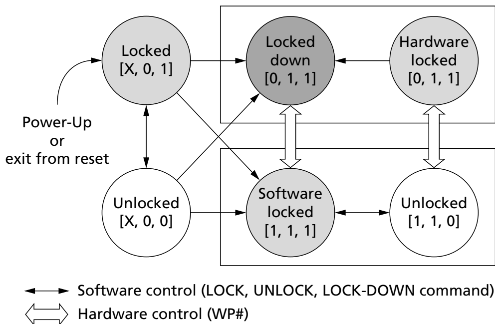
Figure 14: BLOCK LOCK Operations
