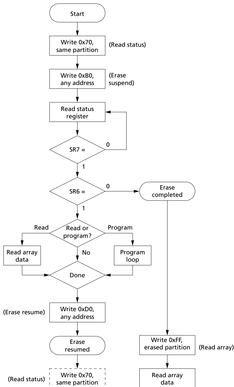
Figure 49: Erase Suspend/Resume Procedure
