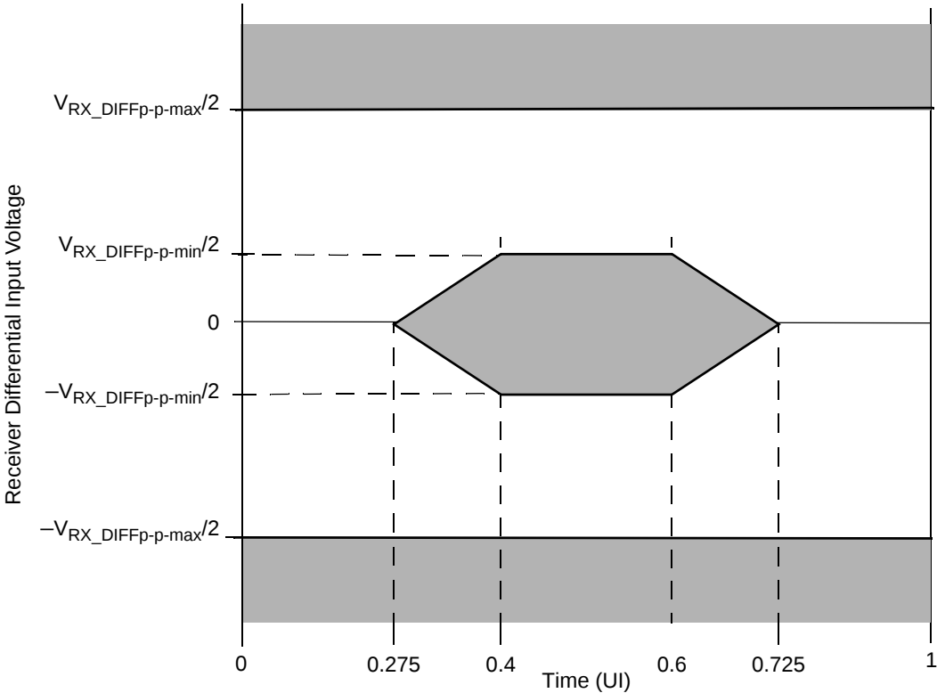
Figure 17. SGMII Receiver Input Compliance Mask
