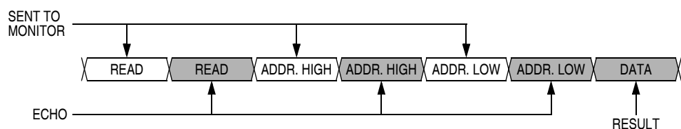
Figure 9-5. Read Transaction
