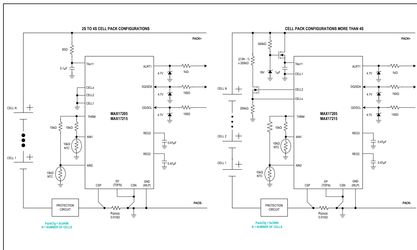
Figure 2. Multicell Schematics
