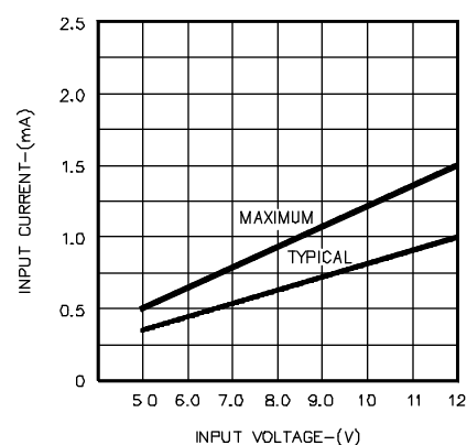
FIGURE 6. INPUT CHARACTERISTICS - SG2804
