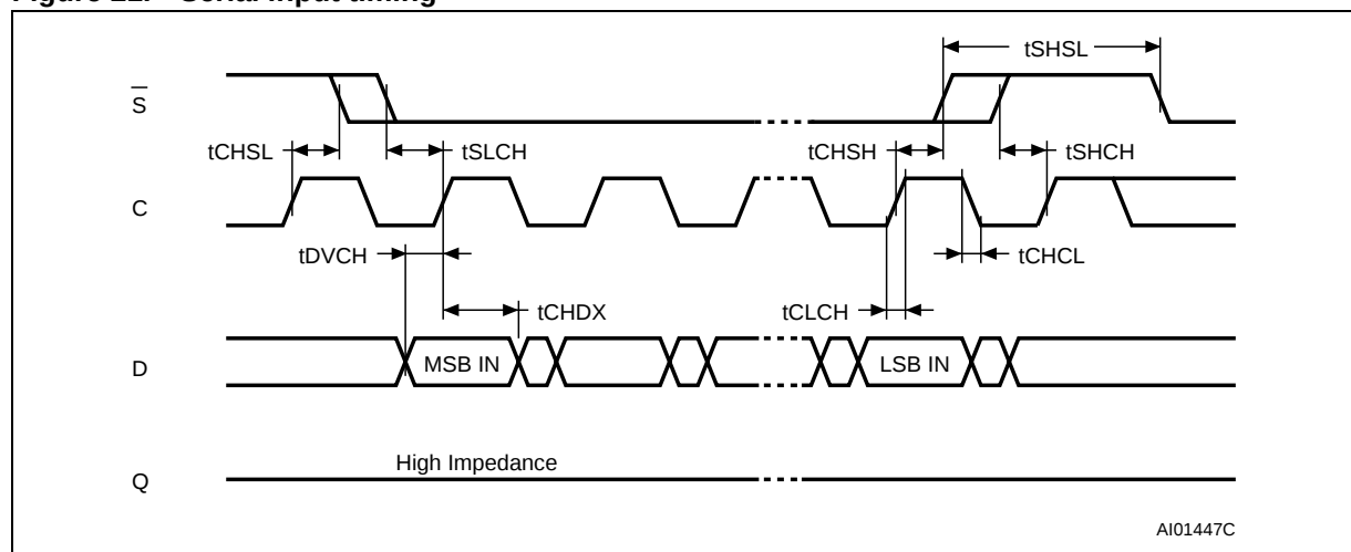
Figure 21. Serial input timing
