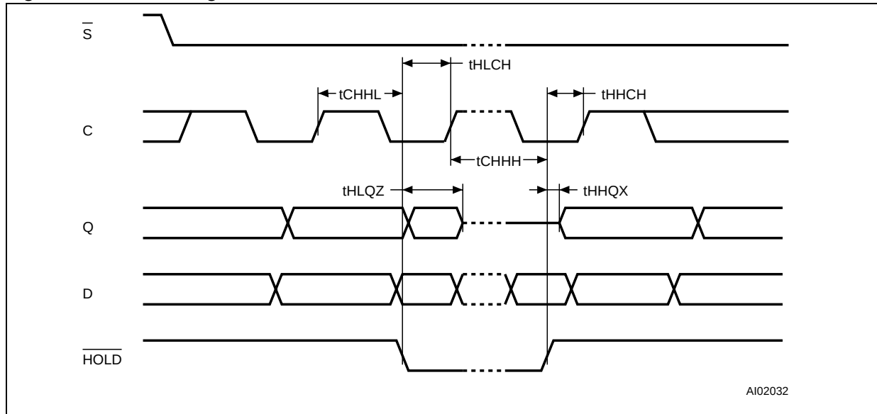
Figure 25. Hold timing
