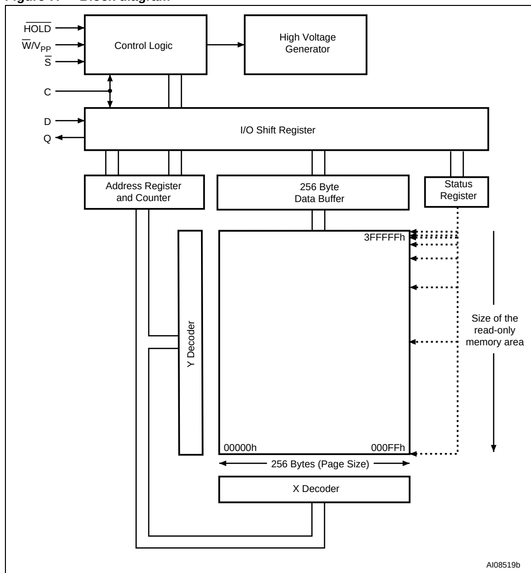
Figure 7. Block diagram
