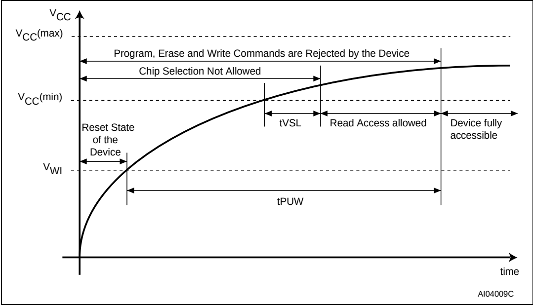
Figure 21. Power-up timing
