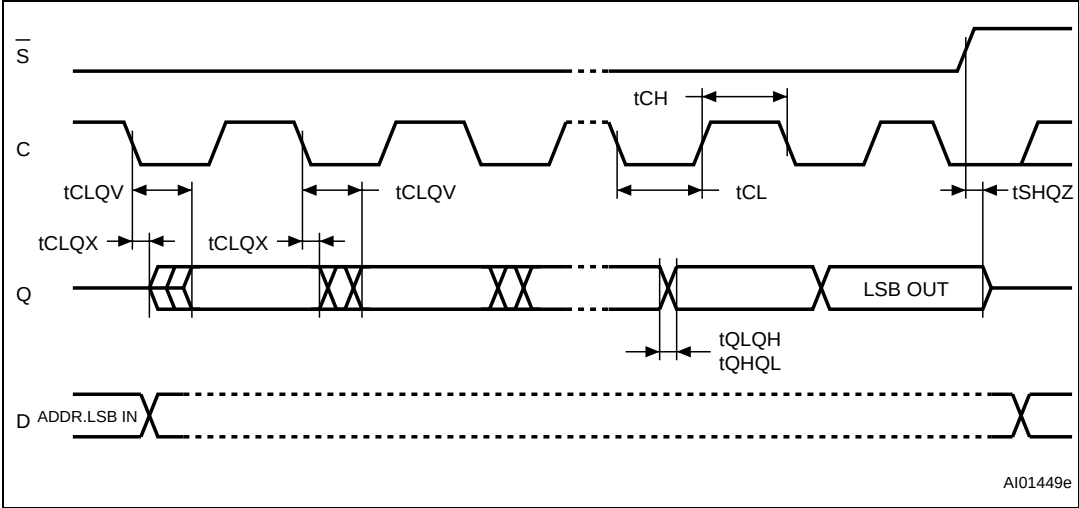
Figure 26. Output timing
