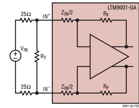
Figure 2. Input Termination for Differential 50Ω Input Impedance Using Shunt Resistor (See Table 2 for R T Values)
