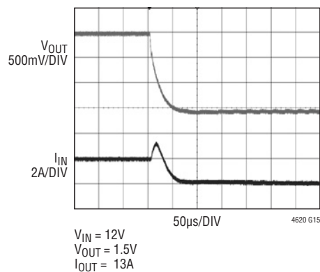
Short-Circuit Protection
