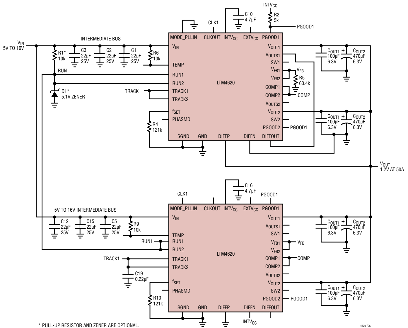
Figure 26. 4-Phase, 1.2V at 50A
