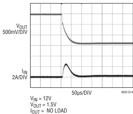
Short-Circuit Protection
