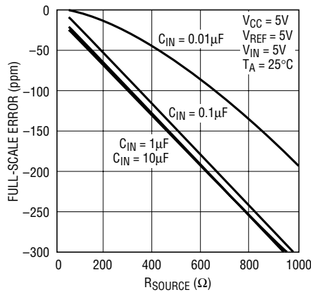
Figure 21. Full-Scale Error vs R_{SOURCE} (Large C)
