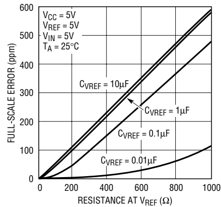
Figure 22. Full-Scale Error vs R_{VREF} (Large C)
