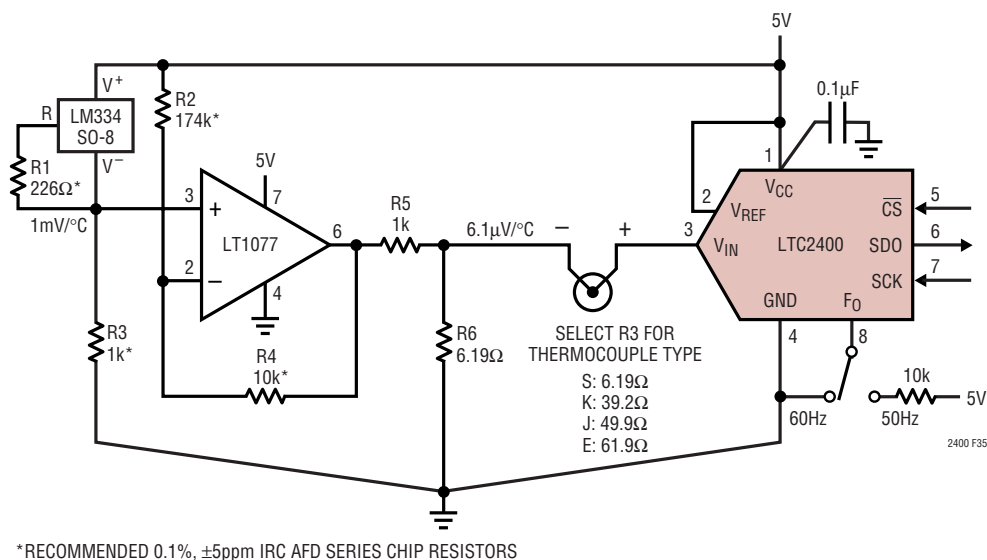
Figure 36. Inexpensive Amplifier Improves Cold Junction Compensation
