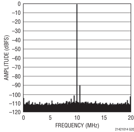
LTC2141-14: 64k Point FFT, f_{IN} = 70\text{MHz} , -1\text{dBFS} , 40\text{MSPS}
