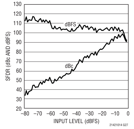
LTC2141-14: SFDR vs Input Level, f_{IN} = 70\text{MHz} , 40\text{MSPS} , 2\text{V} Range
