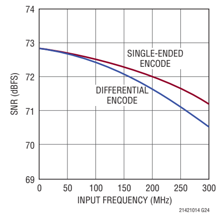
LTC2141-14: SNR vs Input Frequency, -1\text{dBFS} , 105\text{MSPS} , 2\text{V} Range
