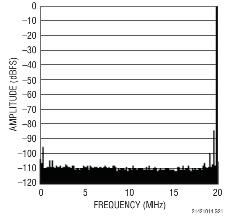
LTC2141-14: 64k Point FFT, f_{IN} = 140\text{MHz} , -1\text{dBFS} , 40\text{MSPS}
