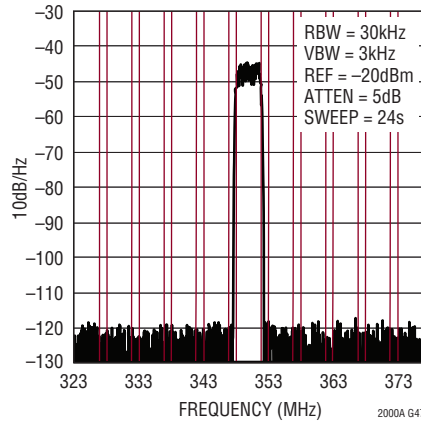
LTC2000A-16 Single Carrier WCDMA ACLR at 350MHz, f_{DAC} = 2.7Gsp/s
