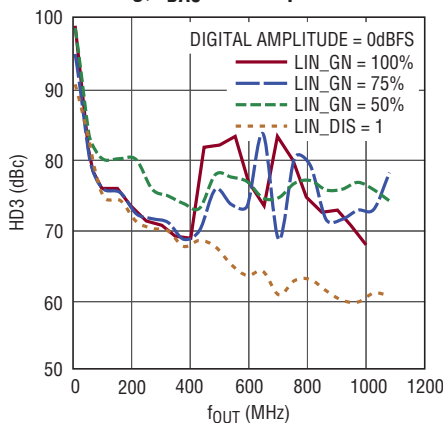
HD3 vs f_{OUT} and Linearization Setting, f_{DAC} = 2.7Gsp/s
