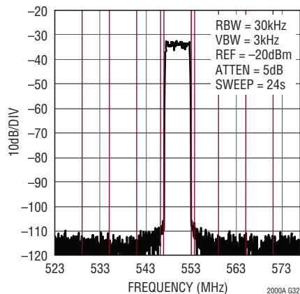
Single Carrier DOCSIS Mid Band Narrowband ACLR, f_{DAC} = 2.7\text{Gsps}
