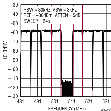
157 Carrier DOCSIS Gap Channel Narrowband ACLR, f_{DAC} = 2.7\text{Gsp/s}
