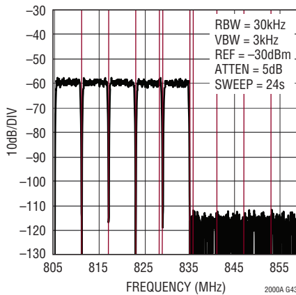
128 Carrier DOCSIS Low Band Narrowband ACLR, f_{DAC} = 2.7\text{Gsp/s}
