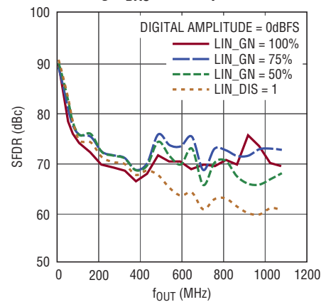
SFDR vs f_{OUT} and Linearization Setting, f_{DAC} = 2.7Gsp/s
