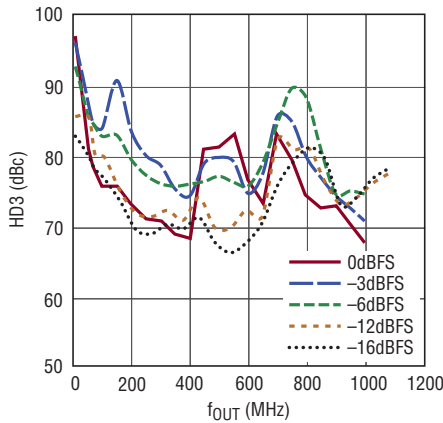
HD3 vs f_{OUT} and Digital Amplitude (dBFS), f_{DAC} = 2.7Gsp/s
