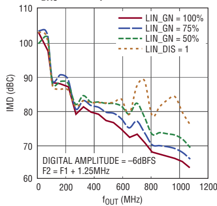
2-Tone IMD vs f_{OUT} and Linearization Setting, f_{DAC} = 2.7Gsp/s
