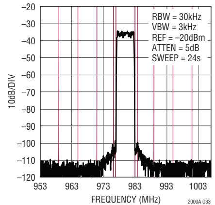
Single Carrier DOCSIS High Band Narrowband ACLR, f_{DAC} = 2.7\text{Gsps}
