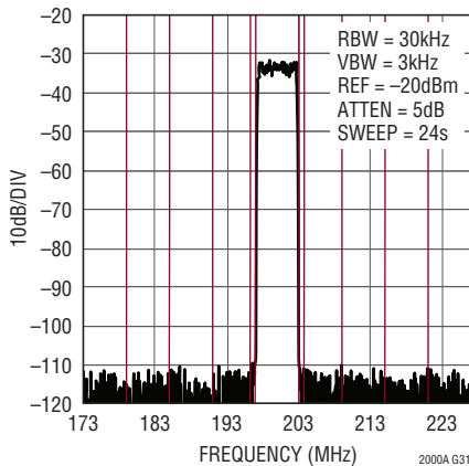
Single Carrier DOCSIS Low Band Narrowband ACLR, f_{DAC} = 2.7\text{Gsps}
