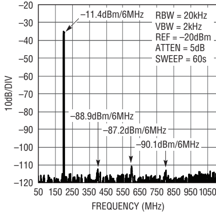
Single Carrier DOCSIS Low Band Wideband ACLR, f_{DAC} = 2.7\text{Gsps}
