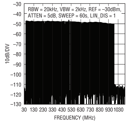
157 Carrier Tones with Gap Channel Wideband ACLR, f_{DAC} = 2.7\text{Gsp/s}
