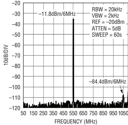
Single Carrier DOCSIS Mid Band Wideband ACLR, f_{DAC} = 2.7\text{Gsps}
