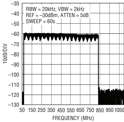
128 Carrier DOCSIS Low Band Wideband ACLR, f_{DAC} = 2.7\text{Gsp/s}
