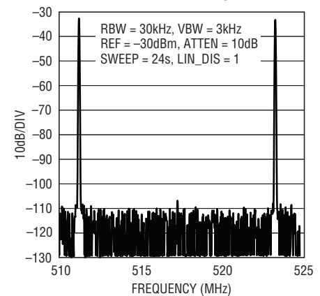
157 Carrier Tones with Gap Channel Narrowband ACLR, f_{DAC} = 2.7\text{Gsp/s}
