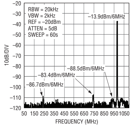
Single Carrier DOCSIS High Band Wideband ACLR, f_{DAC} = 2.7\text{Gsps}
