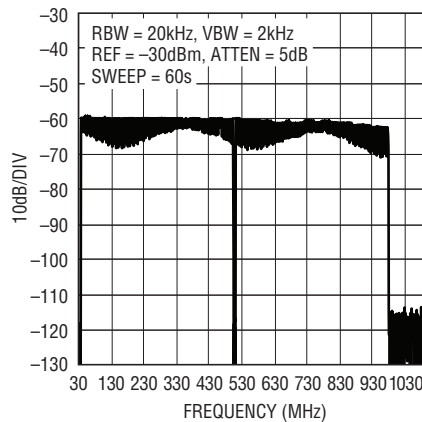
157 Carrier DOCSIS Gap Channel Wideband ACLR, f_{DAC} = 2.7\text{Gsp/s}
