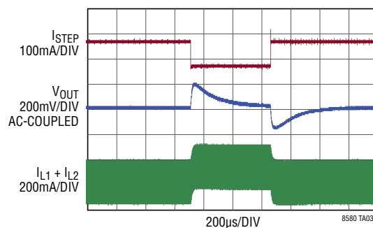
60mA to 160mA to 60mA Output Load Step ( V_{IN} = 12V )
