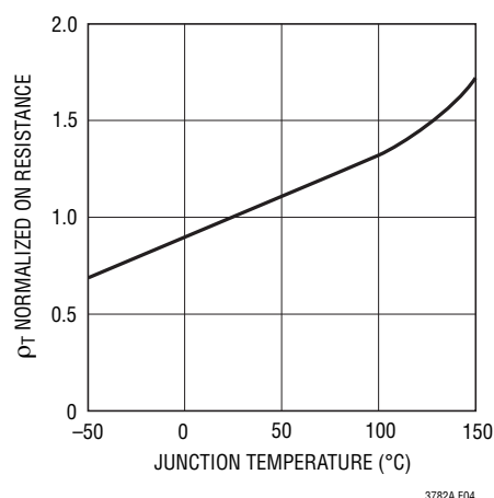
Figure 4. Normalized R_{\text{DS(ON)}} vs Temperature
