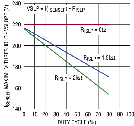
I_{\text{SENSE}} Maximum Threshold – VSLP vs Duty Cycle (Programming Slope Compensation)
