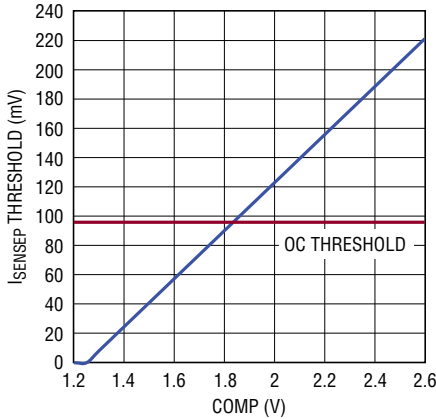
I_{\text{SENSE}} Maximum Threshold vs COMP
