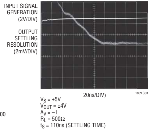
0.01% Settling Time
