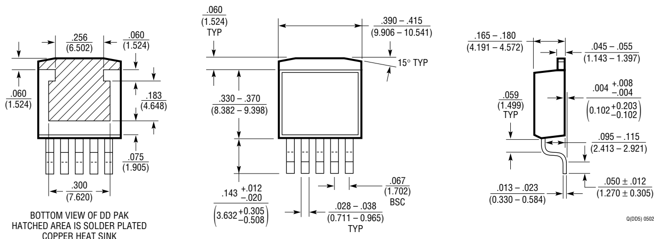
Q Package 5-Lead Plastic DD Pak (Reference LTC DWG # 05-08-1461)
