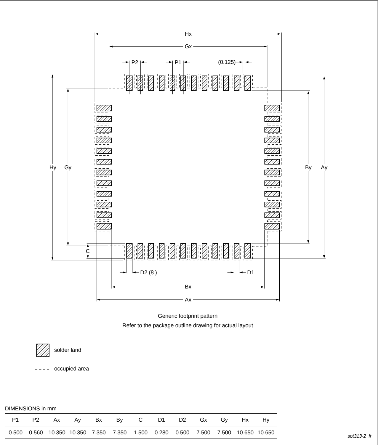
Fig 42. Reflow soldering for the LQFP48 package
