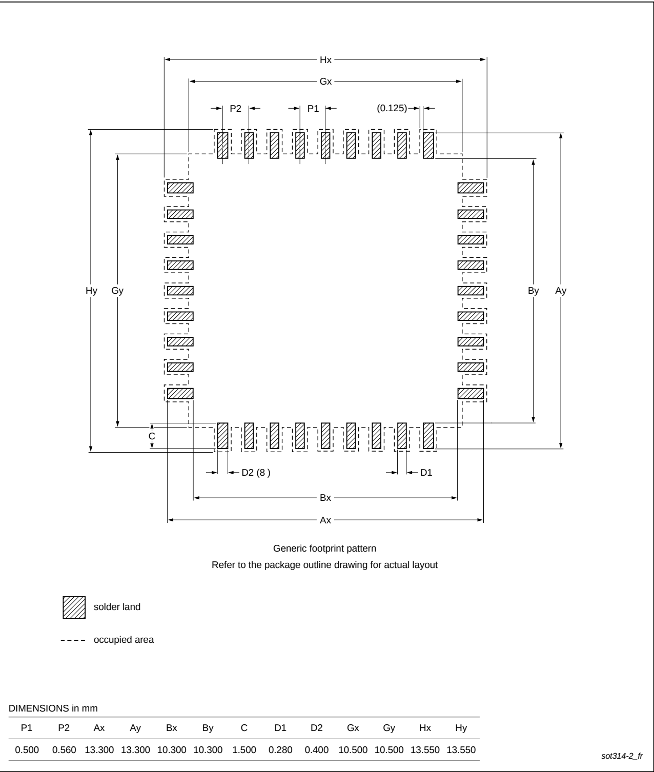
Fig 43. Reflow soldering for the LQFP64 package
